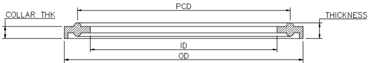
WITH COLLAR
